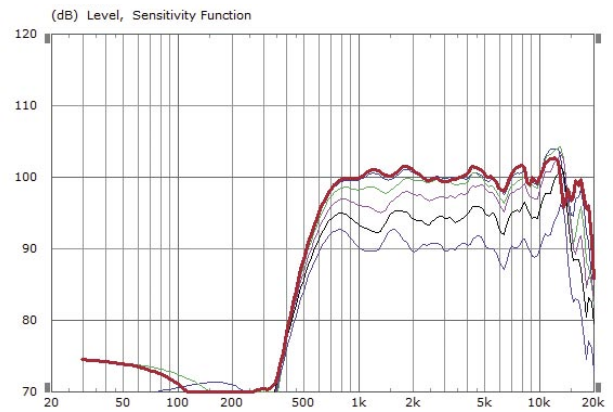
B&C DE920 über passives Filter 0, 10, 20, 30, 40, 50° hor 1/10 oct smoothing
