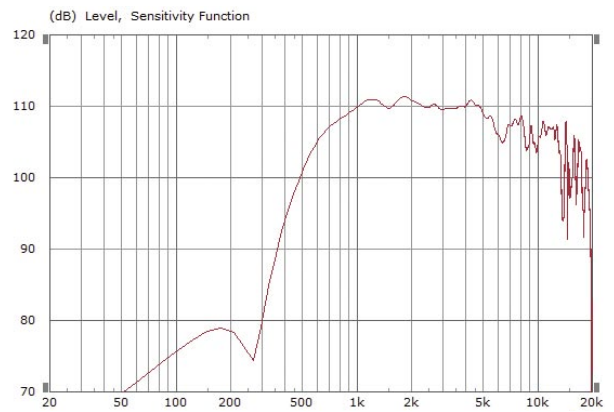
Sensitivity unsmoothed 1W 1m B&C DE920
